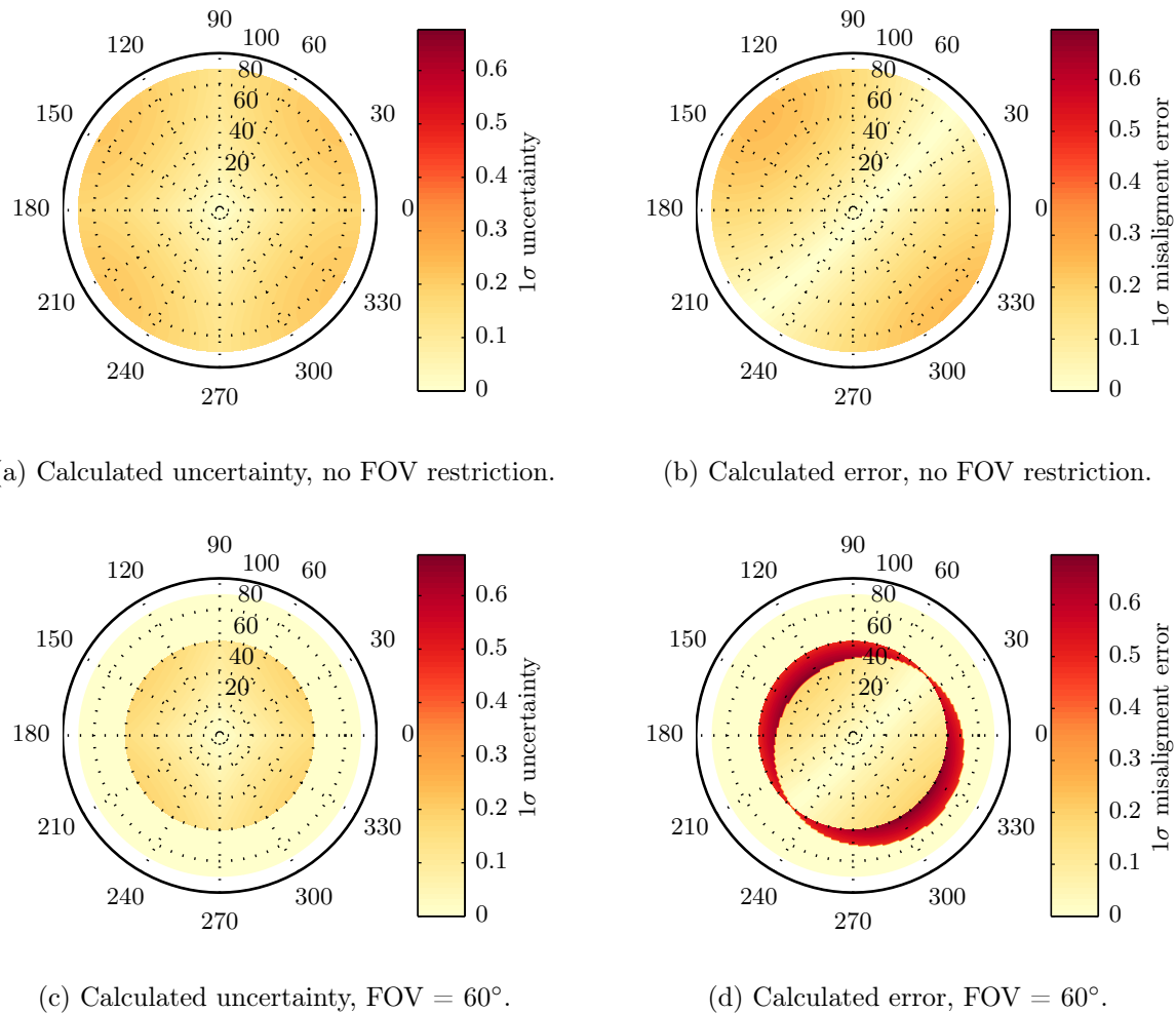
Figure 3.4: Calculated uncertainty and measured error for 1\sigma CSS misalignment.
