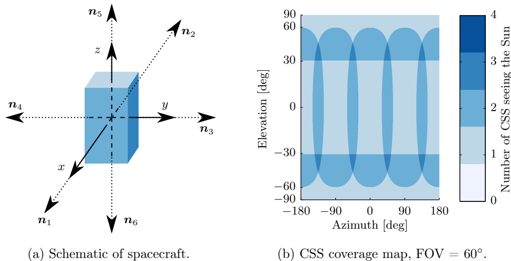
Figure 2.10: Illustration of spacecraft for a simple cube configuration and the associated CSS coverage map.
