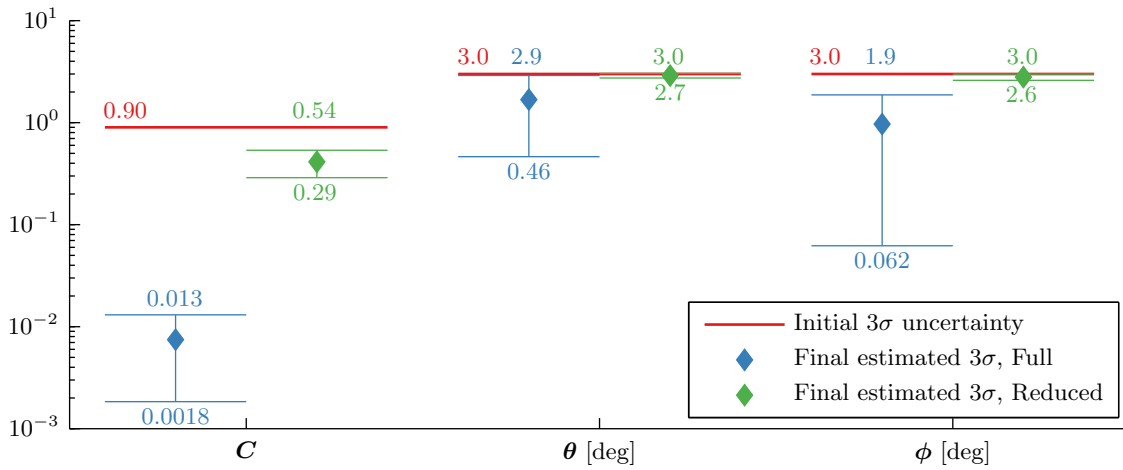
Figure 4.7: Monte Carlo generated statistics of CSS calibration parameter uncertainties for spacecraft using a cube CSS configuration after one orbit.
