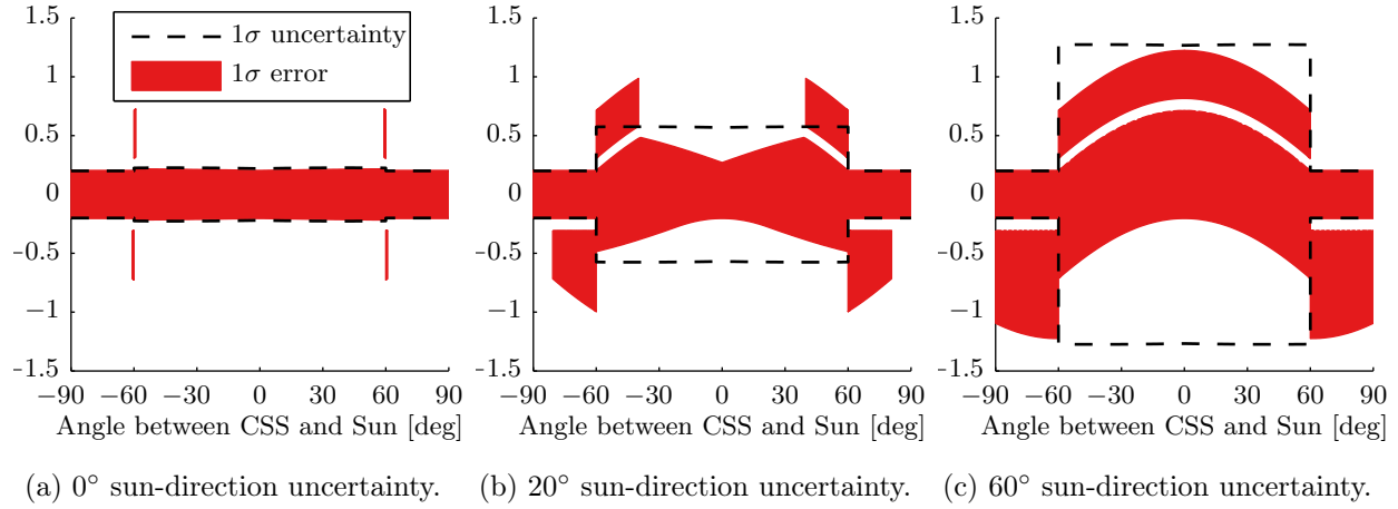
Figure 3.6: 2D slices, through 135° azimuth, of measurement 1\sigma uncertainty and possible errors for 60° FOV.
